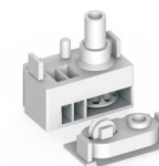
V-001-03R Plastic 塑芯 Control unit 3#制头(右) For 25mm head track Drive-right
