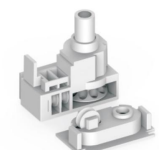
V-001-06R Plastic 塑芯 V-001-06TR Aluminium 铝芯 Control unit 6#制头(右) For 25mm head track Drive-right
